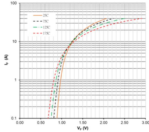
Figure 2. Forward Characteristics
