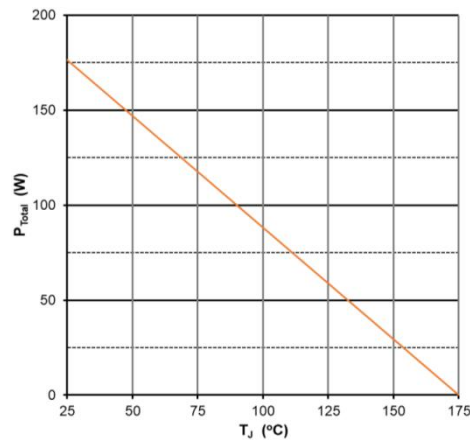
Figure 4. Power Derating
