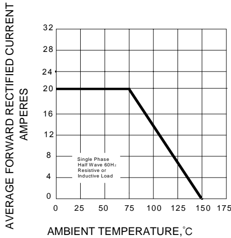
FIG.1 – FORWARD DERATING CURVE
