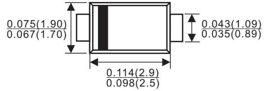
SOD-123FL
