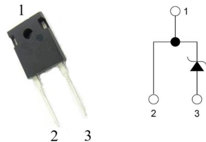
TO-247-2
