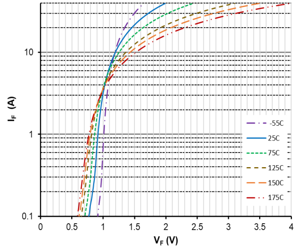
Figure 2. Forward Characteristics
