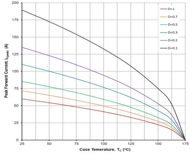
Figure 8. Current Derating
