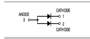
BAT54AW
