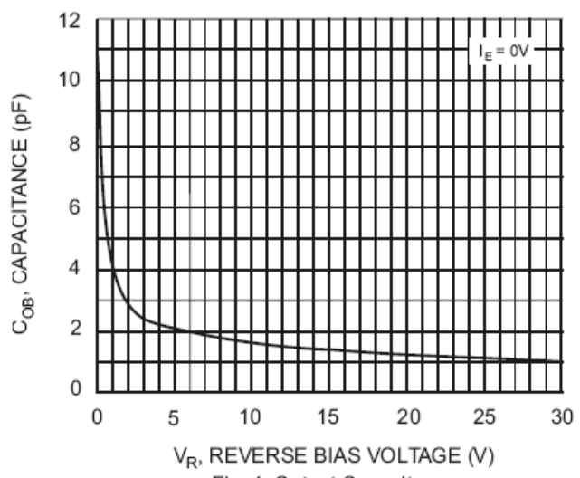
Fig. 4 Output Capacitance
