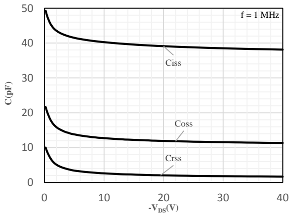
Fig 7 Capacitance Characteristics
