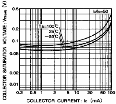
Fig.9 Collector-emitter saturation voltage vs. collector current ( III )
