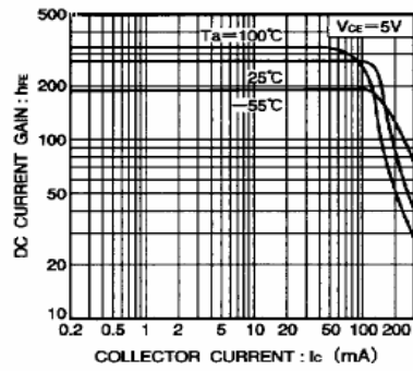
Fig.5 DC current gain vs. collector current ( II )
