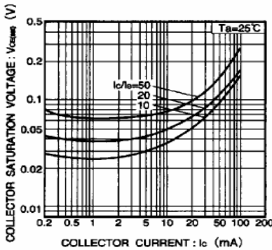
Fig.7 Collector-emitter saturation voltage vs. collector current ( I )
