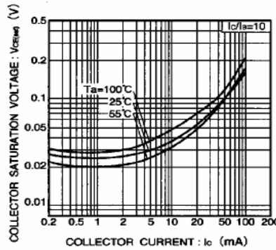
Fig.8 Collector-emitter saturation voltage vs. collector current ( II )
