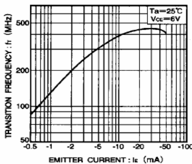
Fig.10 Gain bandwidth product vs. emitter current
