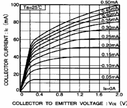
Fig.2 Grounded emitter output characteristics ( I )
