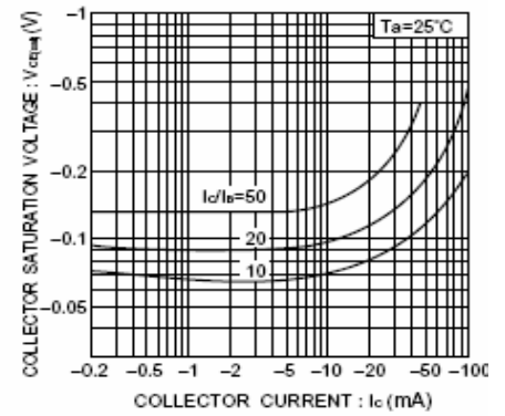
Fig.6 Collector-emitter saturation voltage vs. collector current (I)
