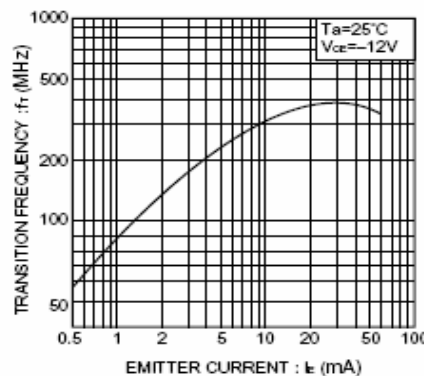
Fig.8 Gain bandwidth product vs. emitter current
