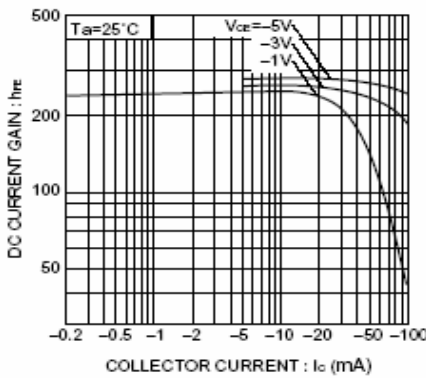
Fig.4 DC current gain vs. collector current (I)
