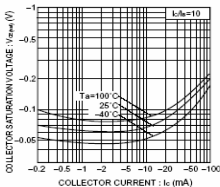
Fig.7 Collector-emitter saturation voltage vs. collector current (II)
