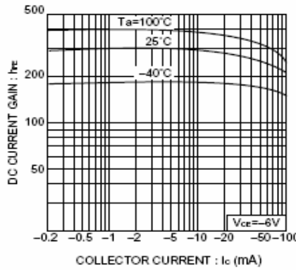
Fig.5 DC current gain vs. collector current (II)
