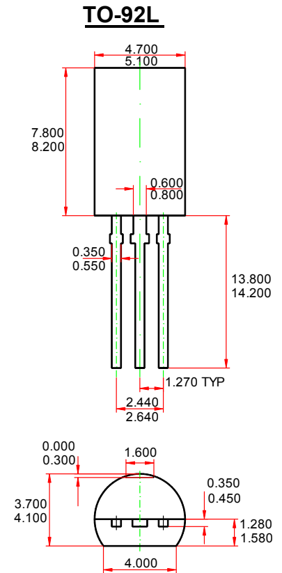
Dimensions in inches and (millimeters)
